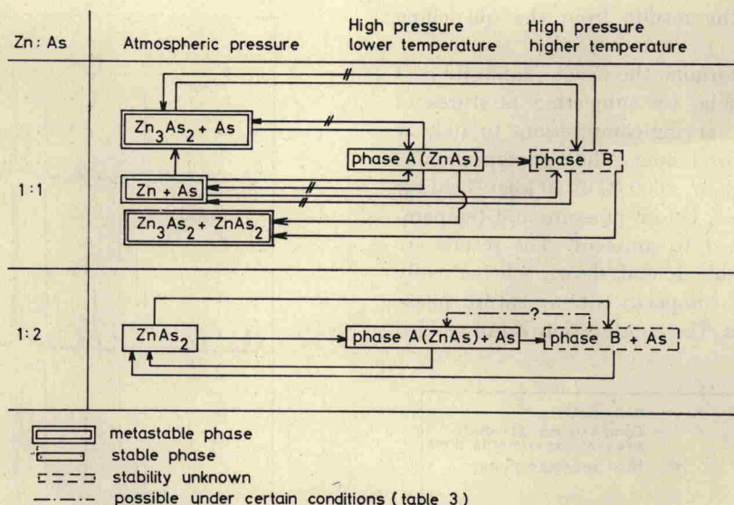
Fig. 4. Stability relationships between phases obtained from high pressures and high temperatures in the \text{Zn}_3\text{As}_2 -As system.
